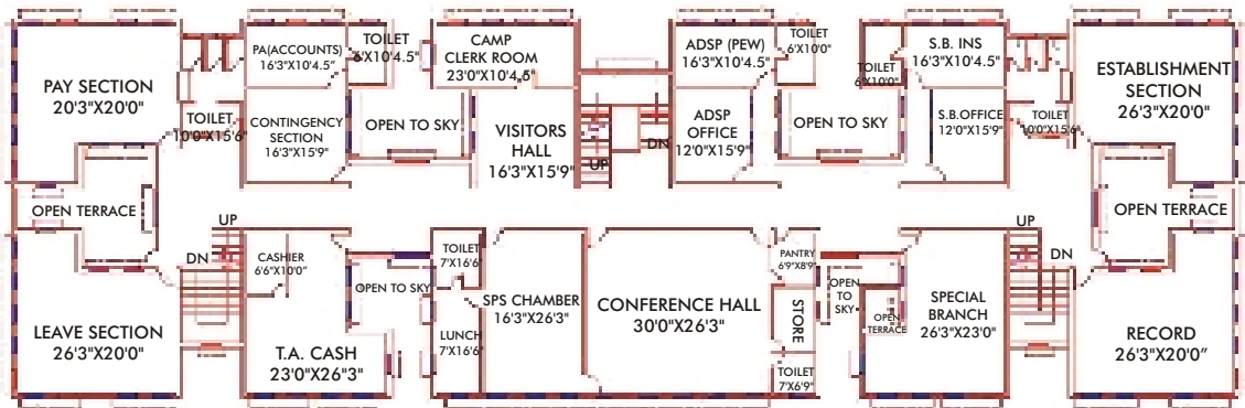
FIRST FLOOR PLAN ( AREA - 10287 sq.ft )
