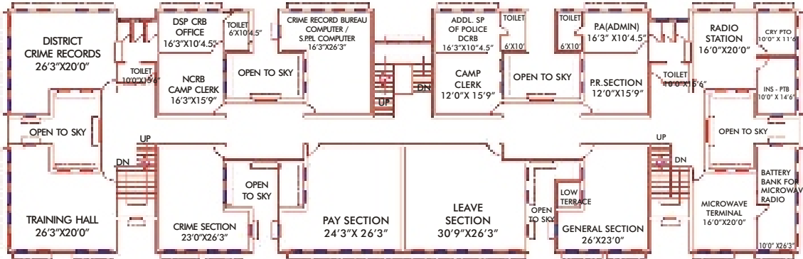
SECOND FLOOR PLAN ( AREA - 10287 sq.ft )
